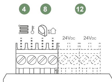
fig. 40 - Raccordements Sondes
