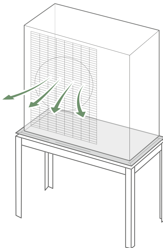
fig. 15 - Support haut (option)
